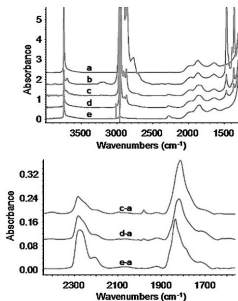
Figure 1. Upper: Transmission IR spectra of: a) KCC-1 treated at 500 °C, b) grafting of [\text{Ta}(=\text{CHtBu})(\text{CH}_2\text{tBu})_3] onto a KCC-1 silica disk. The formation of the tantalum hydride on KCC-1 by treatment under hydrogen (700 mbar) at 150 °C (c), 200 °C (d), and 250 °C (e). Lower: subtracted spectra: c-a, d-a, and e-a.
