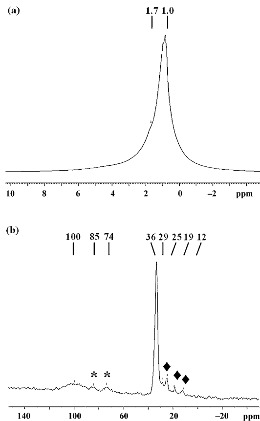
Figure 2. Solid-state NMR spectra of the [\text{Ta}(=\text{CHtBu})(\text{CH}_2\text{tBu})_3]/\text{KCC-1} complex: a) ^1\text{H} MAS spectrum (NS = 64, D1 = 2 s), b) ^{13}\text{C} -CP/MAS spectrum (NS = 30000, D1 = 2 s). * impurities, ♦ traces of remaining template.
